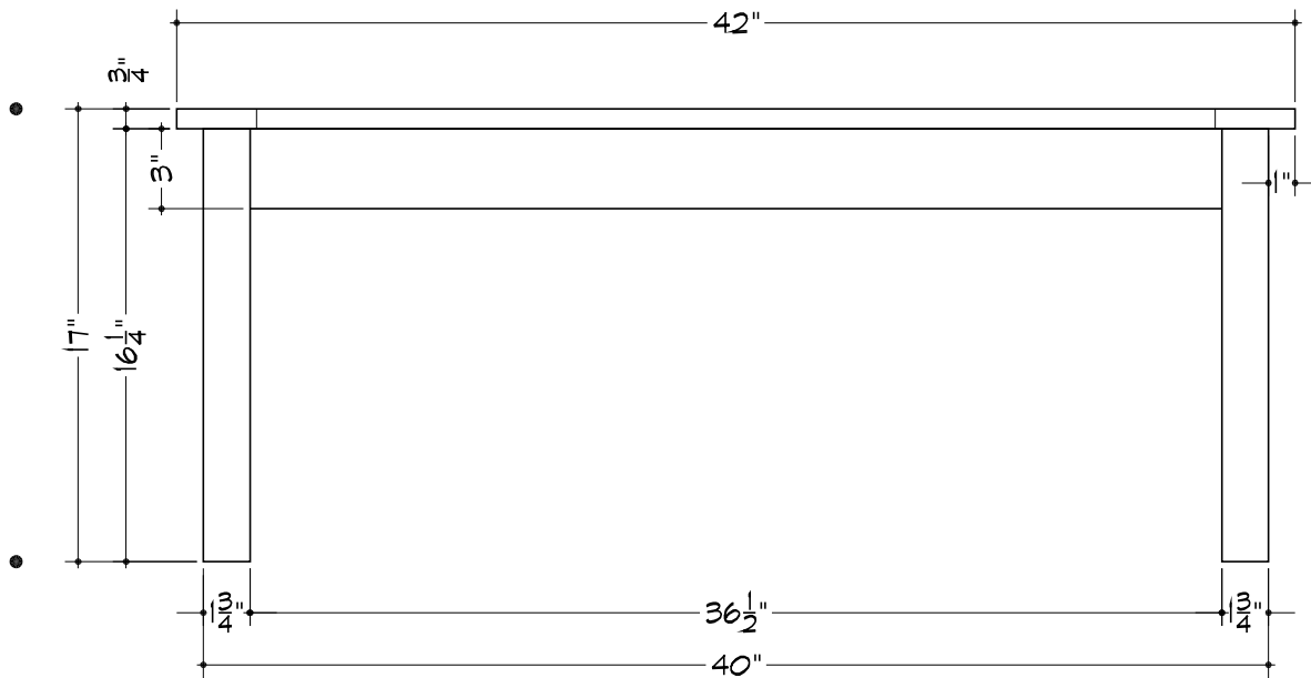
FRONT VIEW
